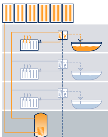
Scheme 5: Two-pipe installation for space heating and hot tap water with centralised solar storage and decentralised backup heaters
