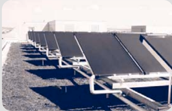
Factory building with solar cooling, Audi, Ingolstadt, Germany
