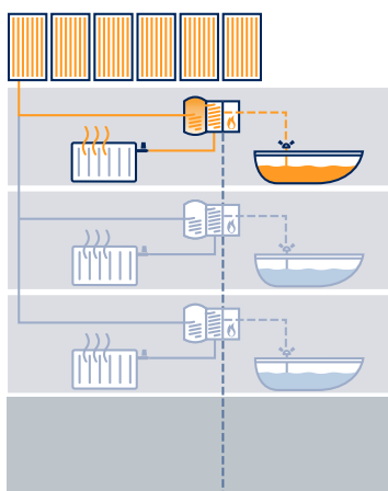
Scheme 4: Direct piping for space heating and hot tap water with decentralised solar storage and backup heaters (common in Spain)
