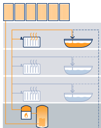
Scheme 6: Two and four-pipe installation for space heating and hot tap water with centralised backup heater and solar buffer (common in D, A, I, DK, NL)
